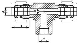
内螺纹支管三通接头T32F BRACH FEMALE TEES FITTING
