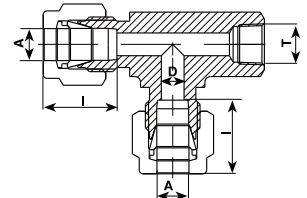
内螺纹三通接头T31F FEMALE TEES FITTING
