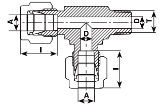
外螺纹三通接头T31 MALE TEES FITTING
