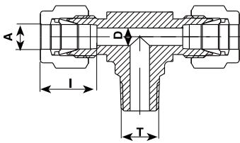
外螺纹支管三通接头T32 BRACH MALE TEES FITTING
